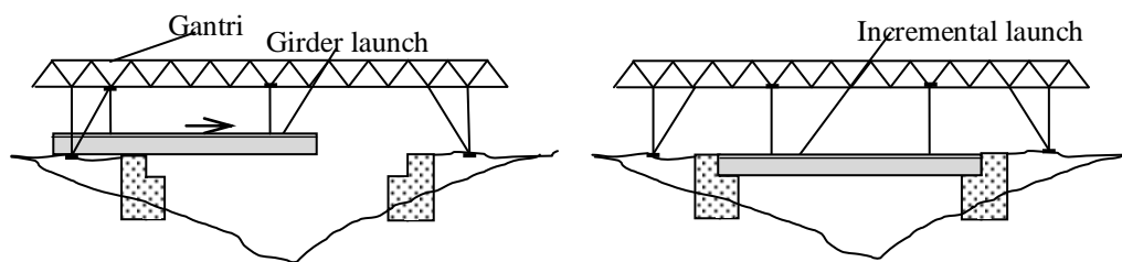
Figure 10. Construction method by girder launch
