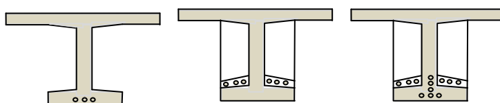
Figure 3. Tendon layout on the girder section
