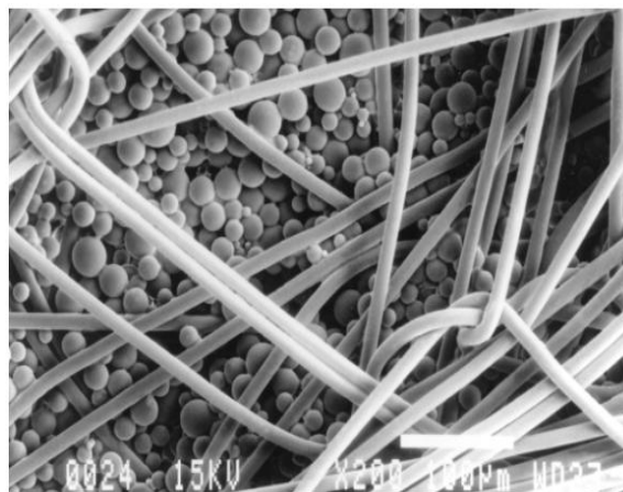
Fig. 4 PCM microcapsules in a fabric (Outlast Europe).
