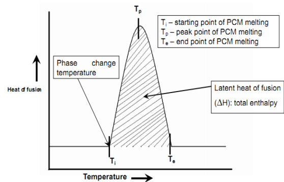
Fig. 3. Schematic of DSC heating thermogram of PCM. [21]
